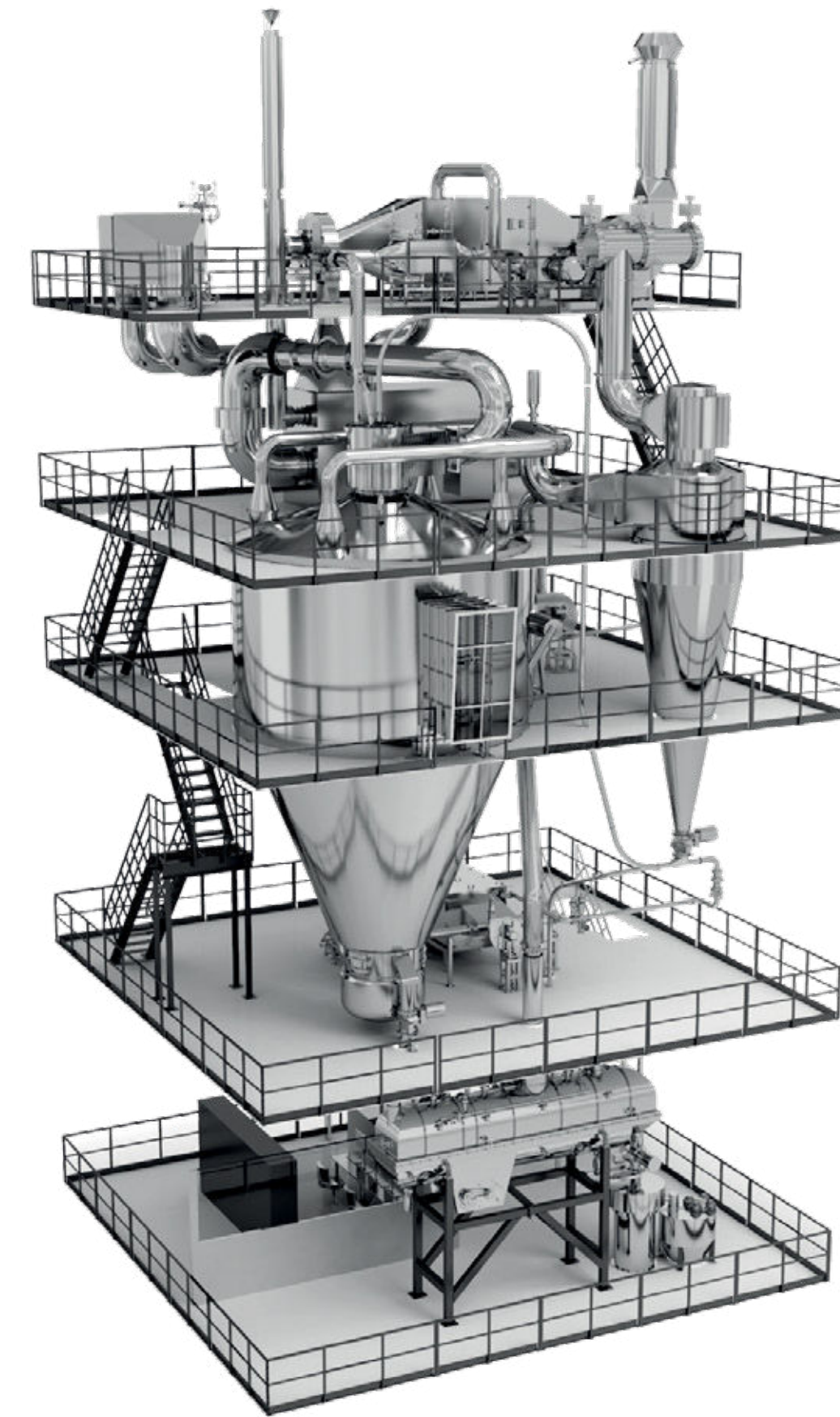
Spray dryer
